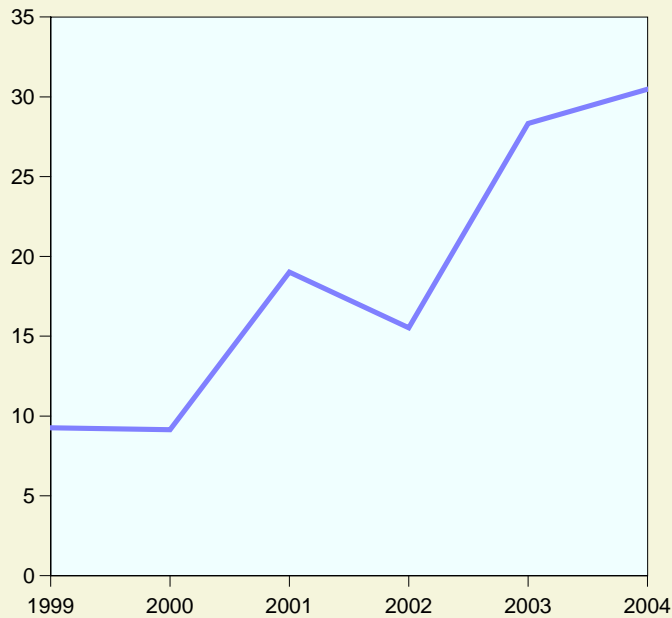
Total Phosphorus
